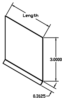
XB03: Optional Horizontal Joint Drip Flashing. For use as closure at horizontal panel joints throughout the system. Available in 10' Lengths.
