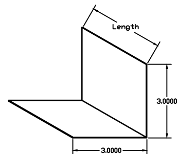
XB04: Optional Inside Corner Closure Flashing. Used for closure at panel to panel inside corners. Available in 10' Lengths.
