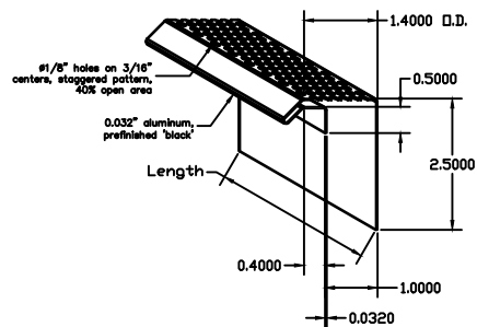
XB01: Optional Top-of-Panel Closure Flashing. Used at panel termination beneath coping, window sills, and other flashings. Available in 10' Lengths.
