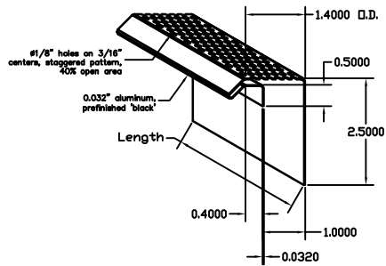
EFB01: Optional Top-of-Panel Closure Flashing. Used at panel termination beneath coping, window sills, and other flashings. Available in 10' Lengths.
