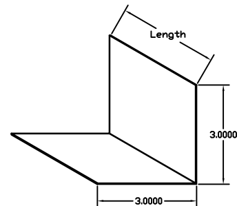
EFB04: Optional Inside Corner Closure Flashing. Used for closure at panel to panel inside corners. Available in 10' Lengths.
