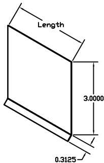
EFB03: Optional Horizontal Joint Flashing. For use as closure at horizontal panel joints throughout the system. Available in 10' Lengths.
